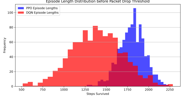
Figure 10. Episode Length Distribution before Packet Drop Threshold.
