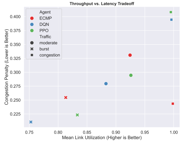
Figure 4. Throughput vs Latency Tradeoff under various scenarios.
